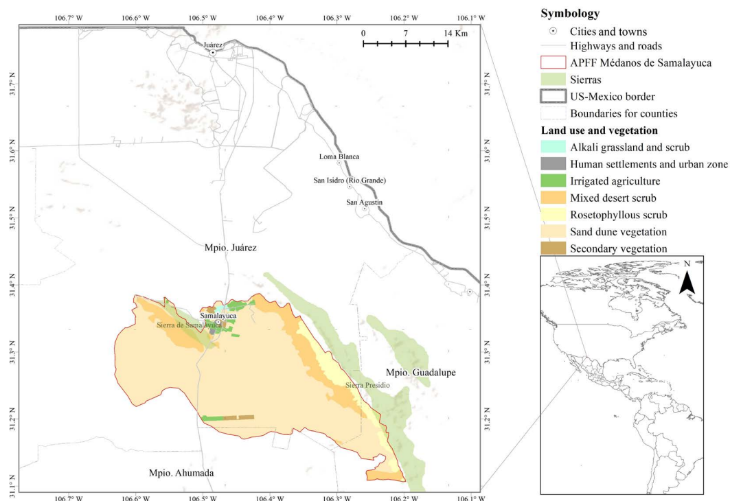
Figure 1. Localization, vegetation types and land use in the Médanos de Samalayuca natural protected area.
